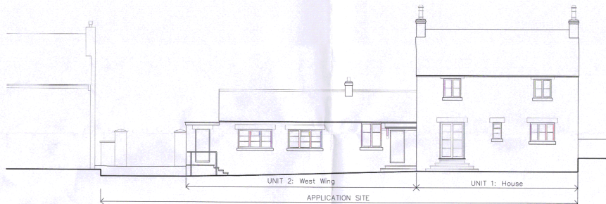
EXISTING SOUTH ELEVATION - UNITS 1 & 2
